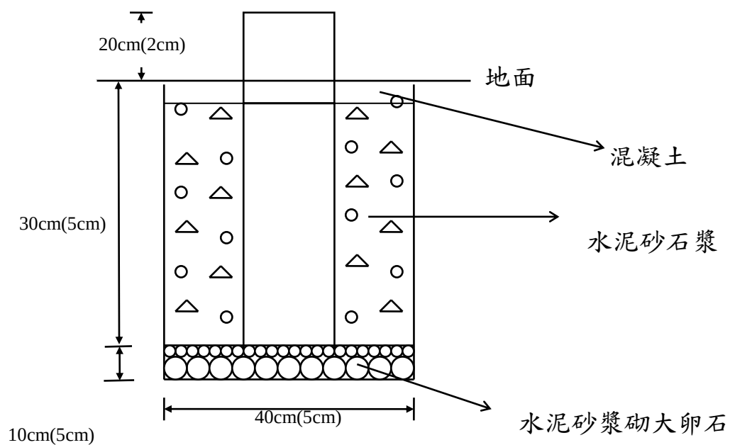
(側視圖)
